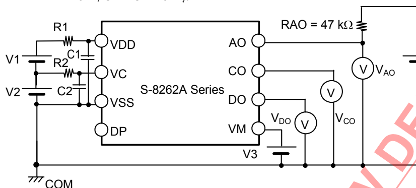
Figure 4 Test Circuit 1
