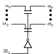
4-Bit Configuration (Configuration 4)
