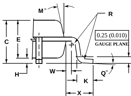
DETAIL AD
