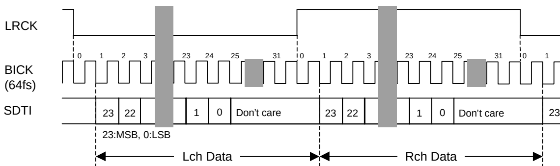
Figure 5. Mode 5 Timing
