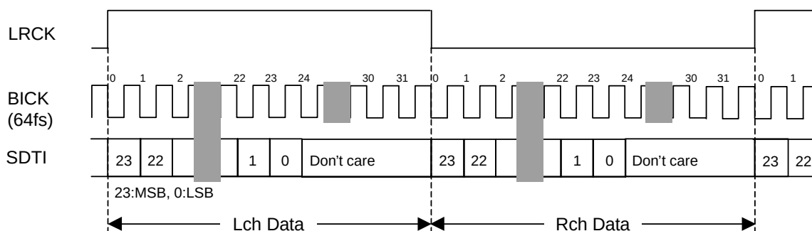
Figure 4. Mode 4 Timing
