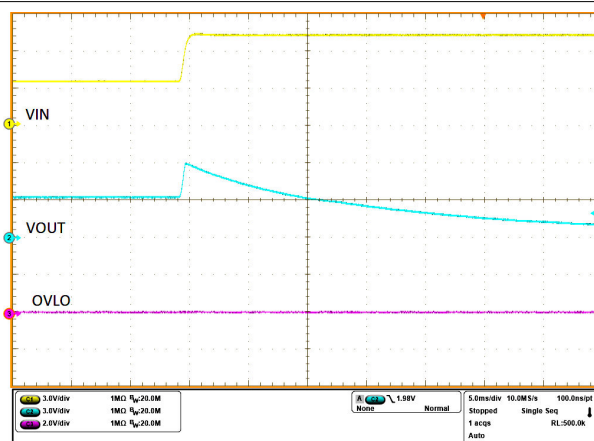
Figure 8-11. Overvoltage protection
