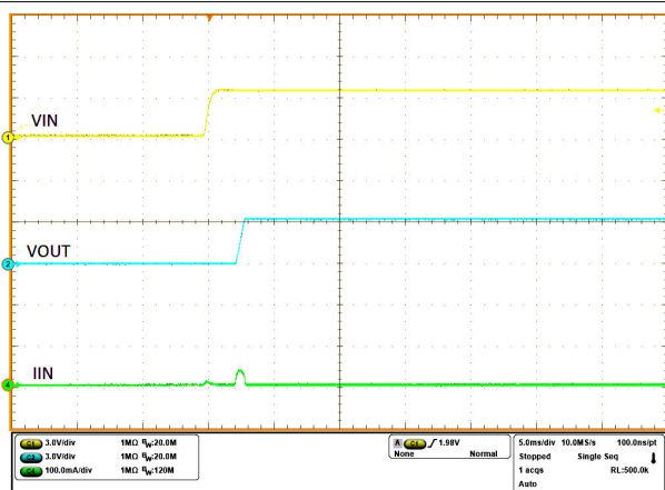
Figure 8-10. Output Ramp
