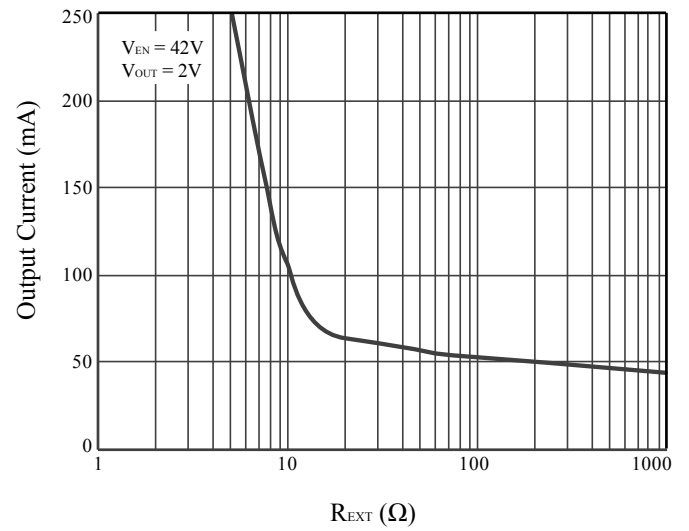
Figure 15 I_{OUT} vs. R_{EXT}
