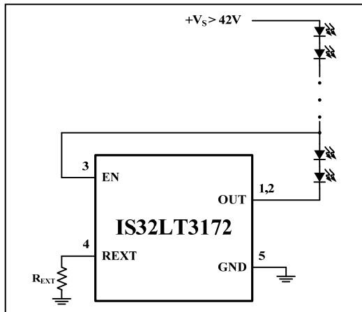
Figure 38 High Input Voltage Application Circuit
