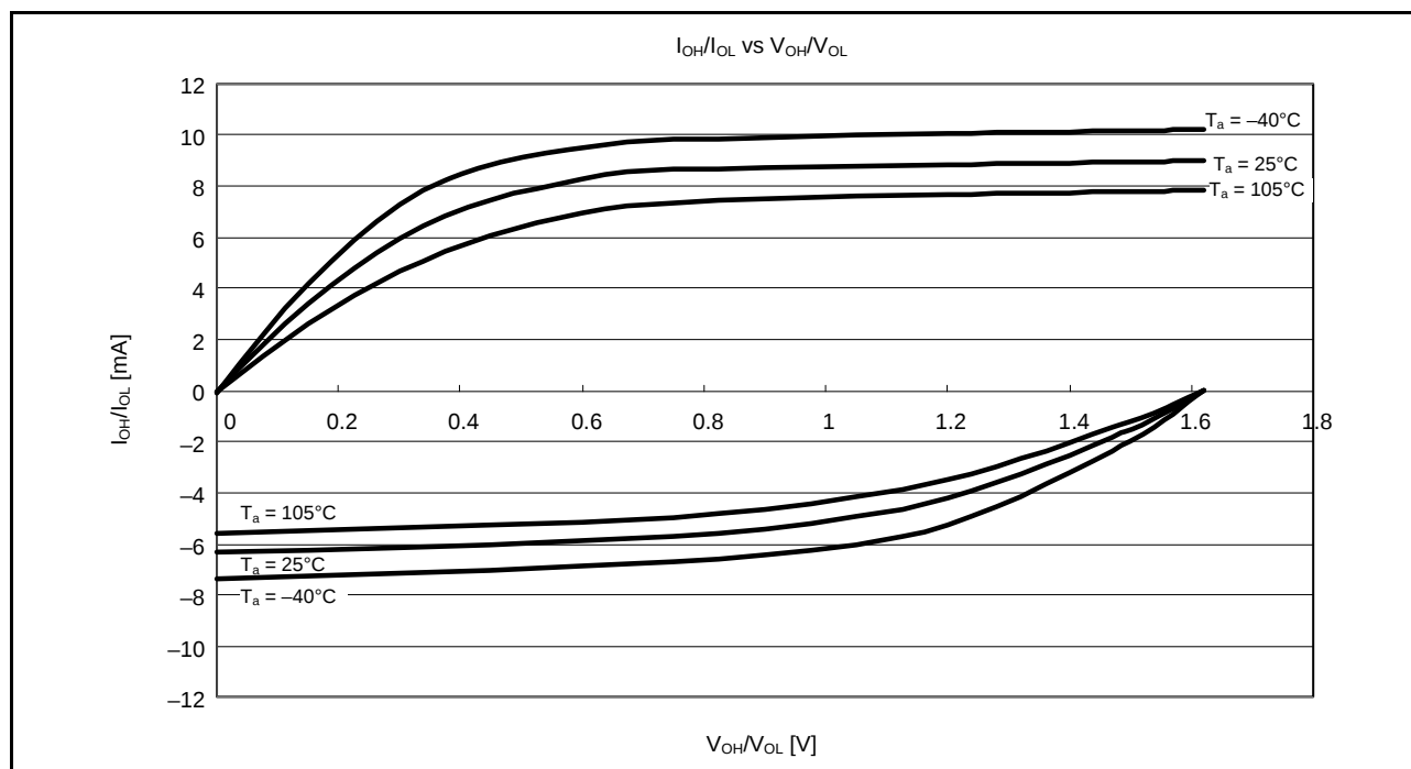
Figure 5.13 V_{OH}/V_{OL} and I_{OH}/I_{OL} Temperature Characteristics at V_{CC} = 1.62 V when High-Drive Output is Selected (Reference Data)
