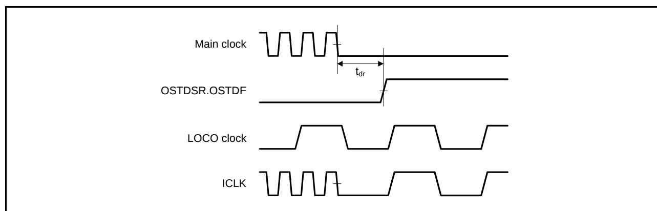
Figure 5.56 Oscillation Stop Detection Timing
