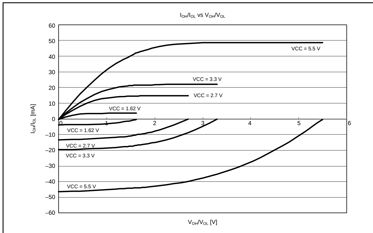
Figure 5.7 V_{OH}/V_{OL} and I_{OH}/I_{OL} Voltage Characteristics at T_a = 25^\circ\text{C} when Normal Output is Selected (Reference Data)
