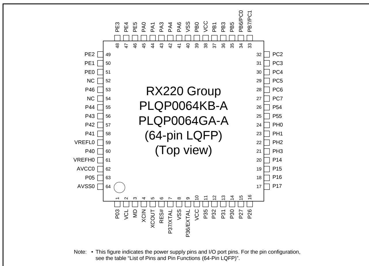
Figure 1.4 Pin Assignments of the 64-Pin LQFP
