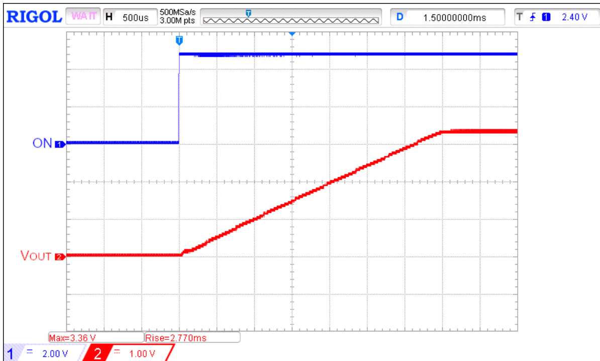
Figure 5. Typical Turn ON operation waveform for V_{DD} = 5\text{ V} , V_{IN} = 3.3\text{ V} , C_{SLEW} = 12\text{ nF} , C_{LOAD} = 10\text{ μF} , R_{LOAD} = 20\text{ Ω}
