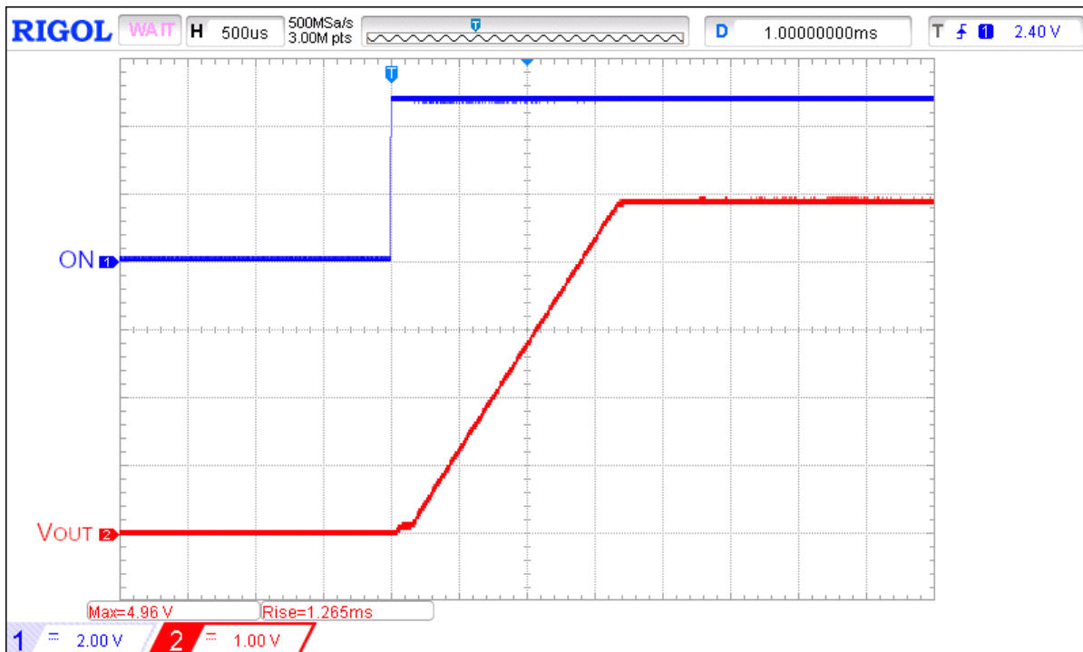
Figure 6. Typical Turn ON operation waveform for V_{DD} = 5\text{ V} , V_{IN} = 5\text{ V} , C_{SLEW} = 3.9\text{ nF} , C_{LOAD} = 10\text{ μF} , R_{LOAD} = 20\text{ Ω}
