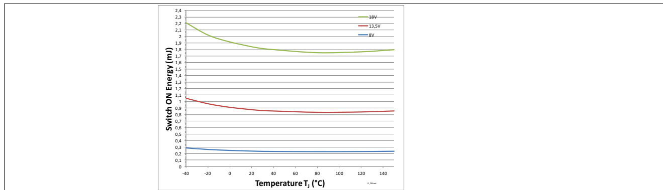
Figure 40 Switch ON Energy E_{ON} = f(T_J; V_{GS}) , R_L = 2 \Omega
