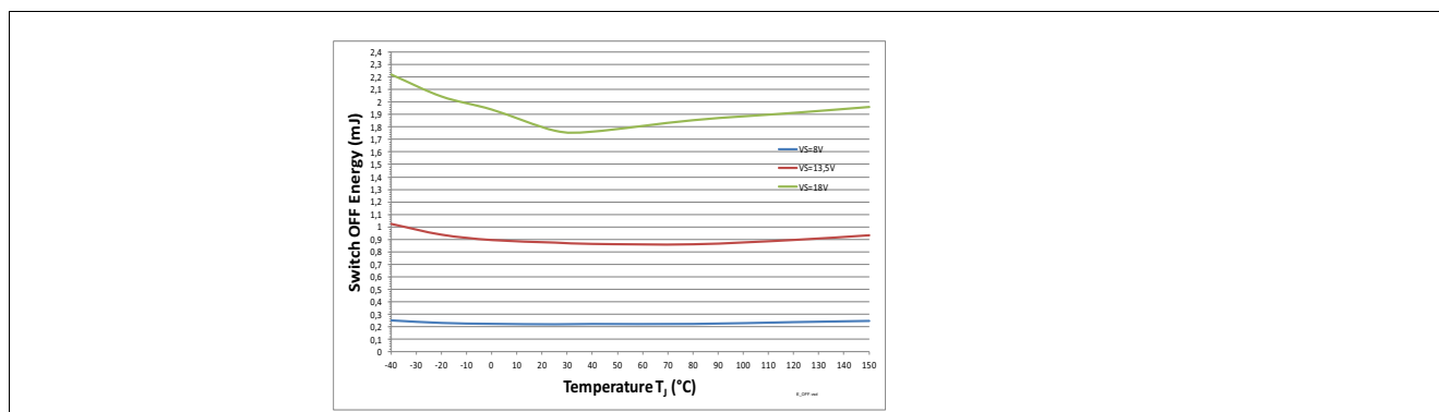
Figure 41 Switch OFF Energy E_{OFF} = f(T_J; V_{DS}) , R_L = 2 \Omega
