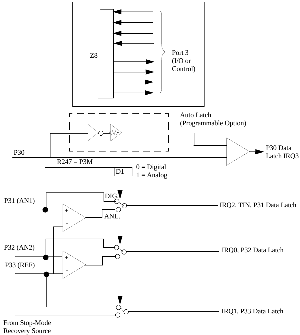
Figure 5. Port 3 Configuration
