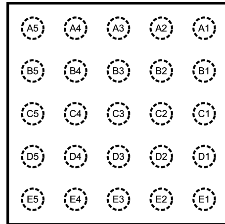
MicroSMD Bottom View
