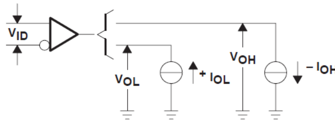
Figure 6-2. Receiver V_{OH} and V_{OL}
