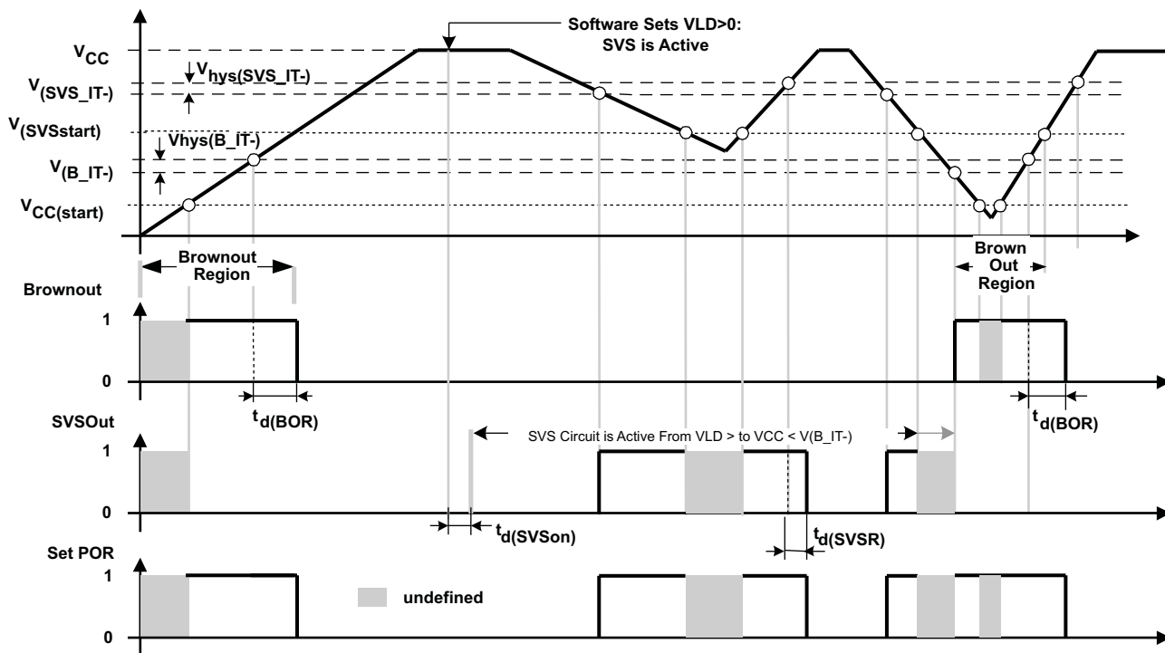
Figure 5-10. SVS Reset (SVSR) vs Supply Voltage
