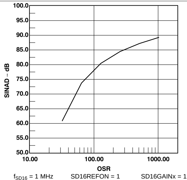
Figure 5-19. SINAD Performance vs OSR
