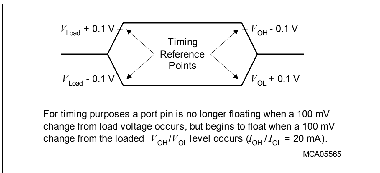
Figure 18 Float Waveforms
