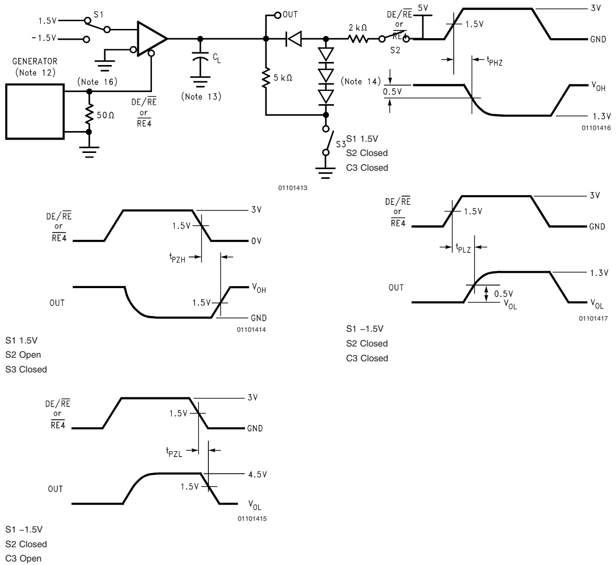
FIGURE 8. Receiver Enable and Disable Timing
