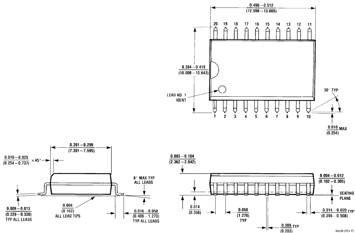
Order Number DS36954M NS Package Number M20B
