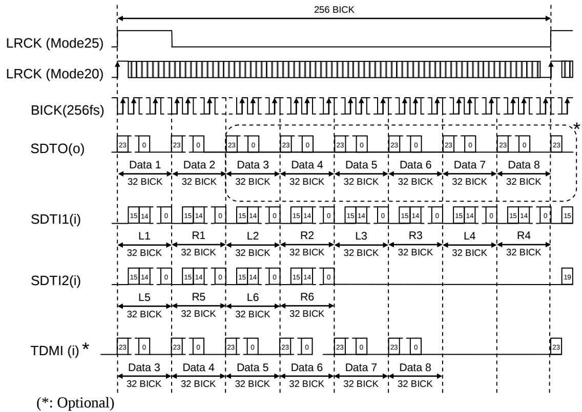
Figure 26. Mode 20/25 Timing (TDM256 Mode)
