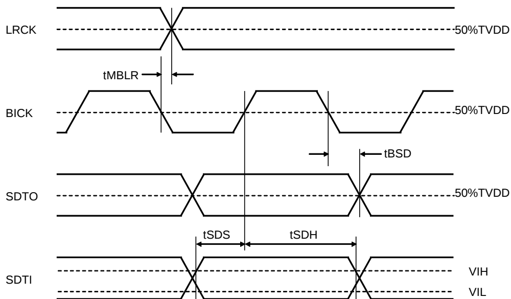
Figure 8. Audio Interface Timing (TDM1-0 bit = "00" &amp; Master mode)
