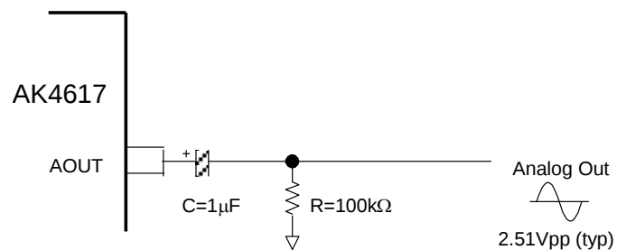
Figure 57. External Circuit Example (LOUT1-6, ROUT1-6 pins)
