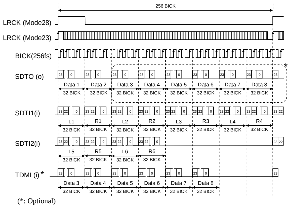
Figure 29. Mode 23/28 Timing (TDM256 Mode)
