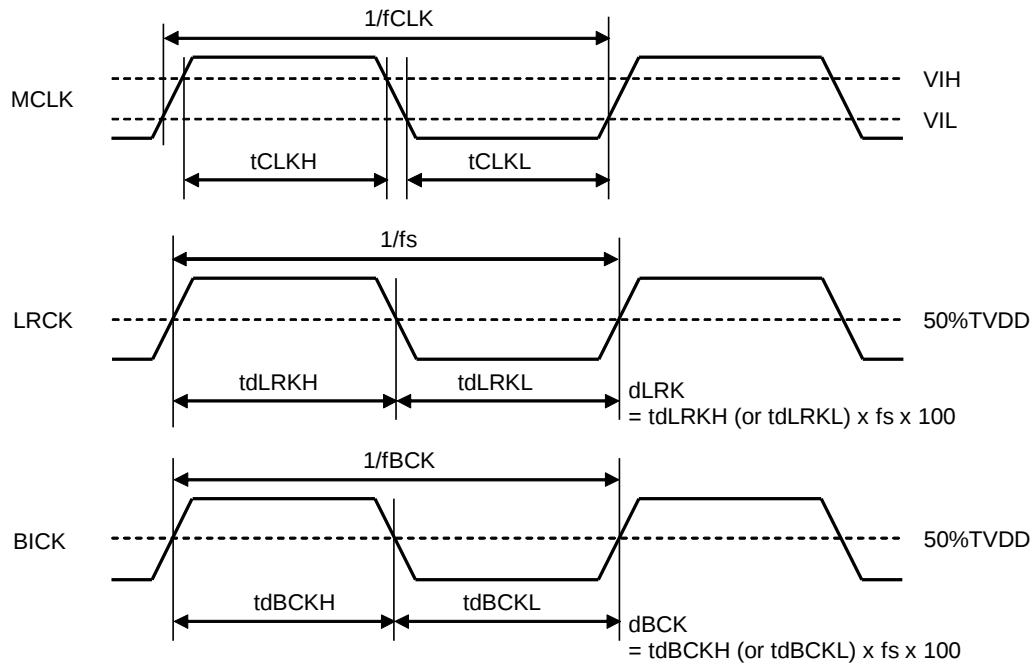
Figure 4. Clock Timing (TDM1-0 bit = "00" &amp; Master mode)
