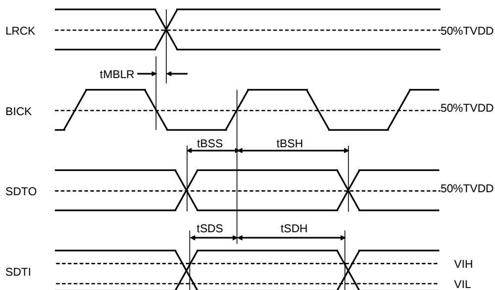
Figure 9. Audio Interface Timing (Except TDM1-0 bit = "00" &amp; Master mode)
