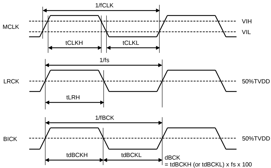
Figure 5. Clock Timing (Except TDM1-0 bit = "00" &amp; Master mode)
