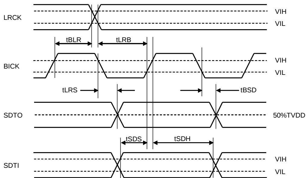
Figure 6. Audio Interface Timing (TDM1-0 bit = "00" &amp; Slave mode)
