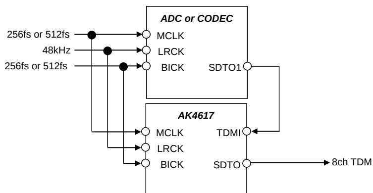
Figure 36. Cascade TDM Connection Diagram
