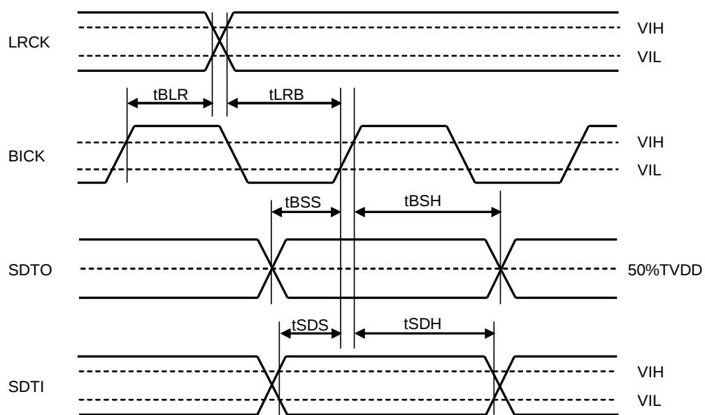
Figure 7. Audio Interface Timing (Except TDM1-0 bit = "00" &amp; Slave mode)
