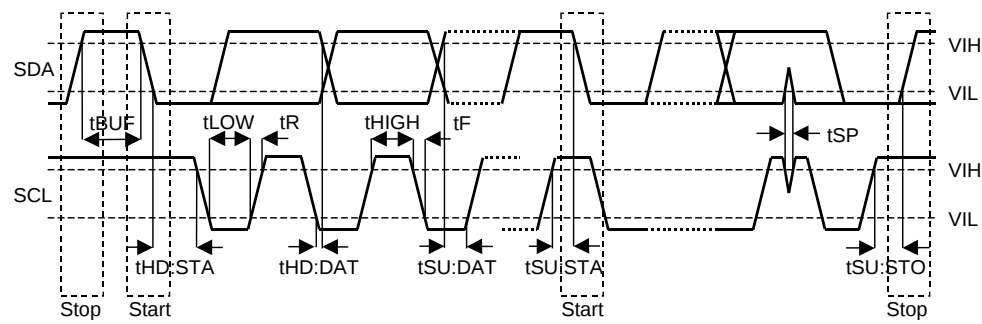
Figure 14. I²C Bus mode Timing
