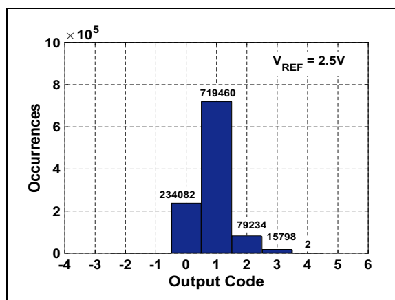
FIGURE 3-29: Shorted Input Histogram: V_{REF} = 2.5\text{V} .
