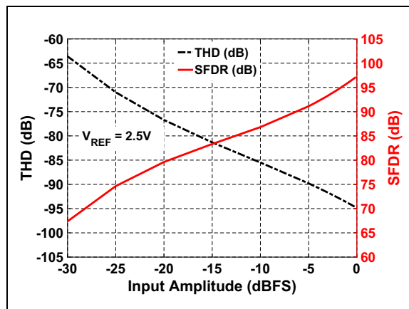
FIGURE 3-28: THD/SFDR vs. Input Amplitude: V_{REF} = 2.5\text{V} .
