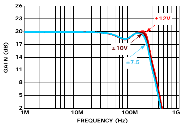
FIGURE 36. SMALL SIGNAL BANDWIDTH vs SUPPLY VOLTAGE
