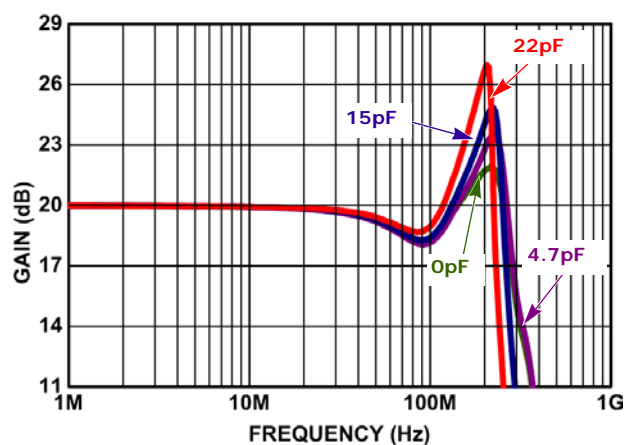
FIGURE 20. SMALL SIGNAL FREQUENCY RESPONSE vs C_{LOAD}
