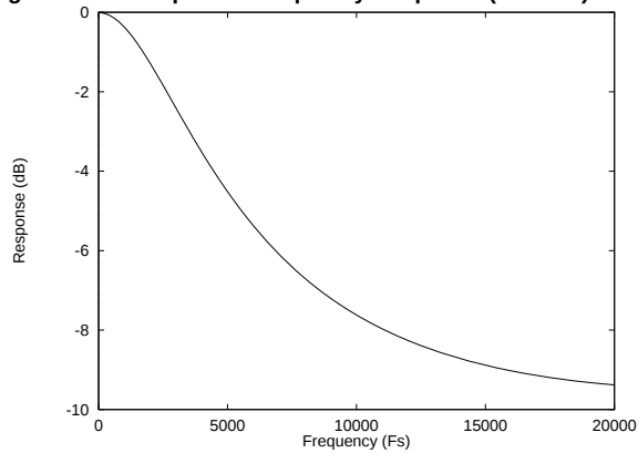
Figure 48 De-emphasis Frequency Response (48kHz)
