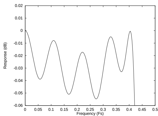
Figure 28 DAC Digital Filter Frequency Response – Type 0
