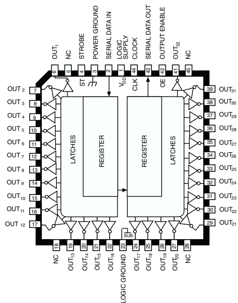
Pin-out Diagram
