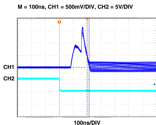
FIGURE 19. ENABLED RESPONSE
