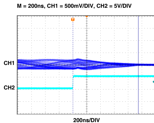
FIGURE 20. DISABLED RESPONSE
