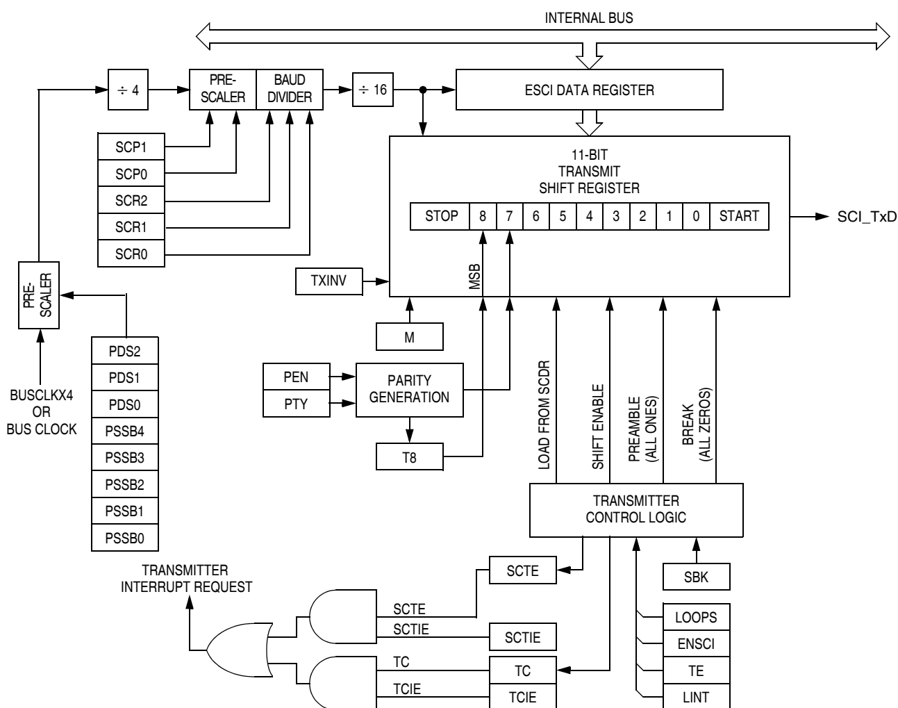
Figure 13-4. ESCI Transmitter
