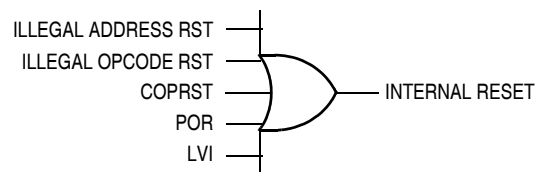
Figure 14-5. Sources of Internal Reset
