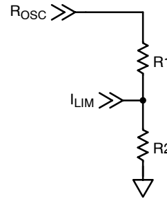
Figure 37. Programming the Current Limit
