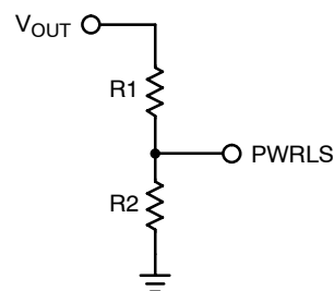
Figure 22. Adjusting the PWRGD Threshold
