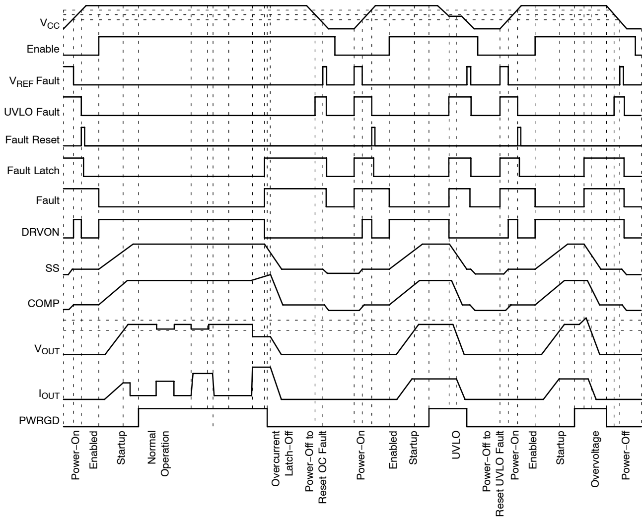
Figure 16. Operating Waveforms
