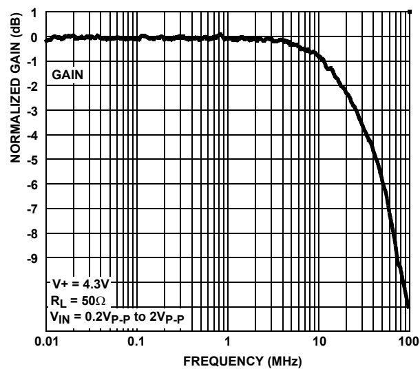
FIGURE 21. FREQUENCY RESPONSE
