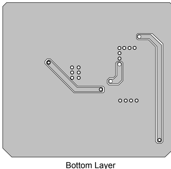
Figure 3: Boost PCB Layout
