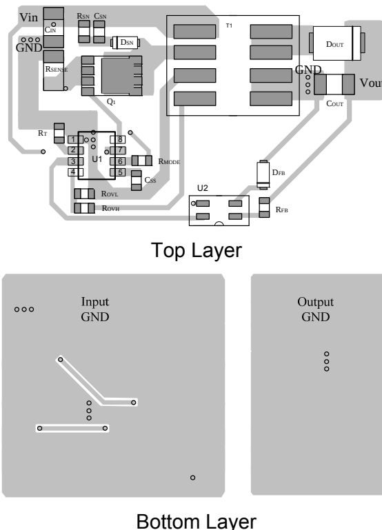
Figure 4: Fly-back PCB Layout
