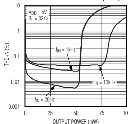
TOTAL HARMONIC DISTORTION PLUS NOISE vs. OUTPUT POWER (UCSP)
