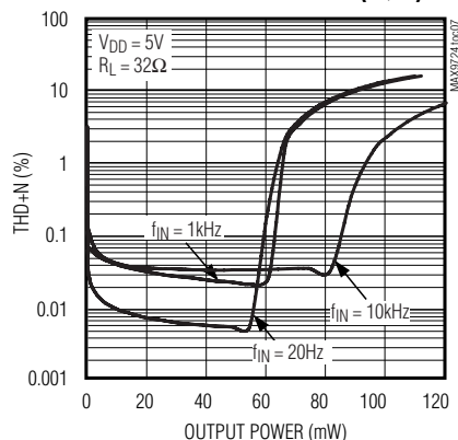
TOTAL HARMONIC DISTORTION PLUS NOISE vs. OUTPUT POWER (TQFN)
