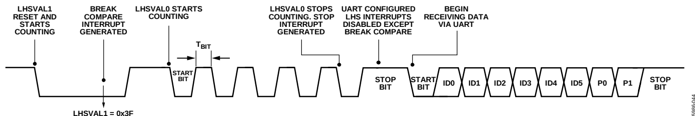
Figure 46. Example LIN Configuration
