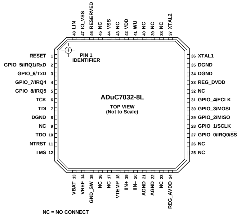
Figure 8. Pin Configuration
