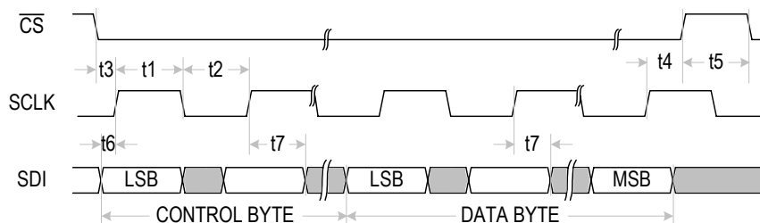
Figure-25 Serial Interface Write Timing
