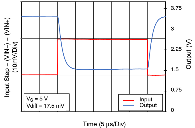
Figure 21c. Small Signal Step Response Inverting, G200
