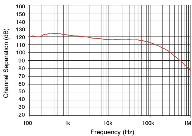
Figure 26. Channel Separation, G 200
