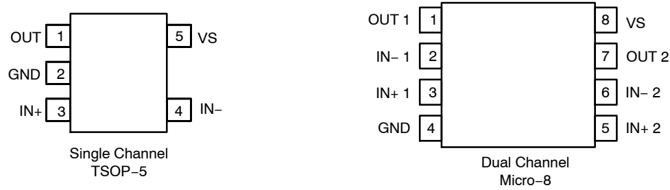
Figure 2. Pin Function Description
