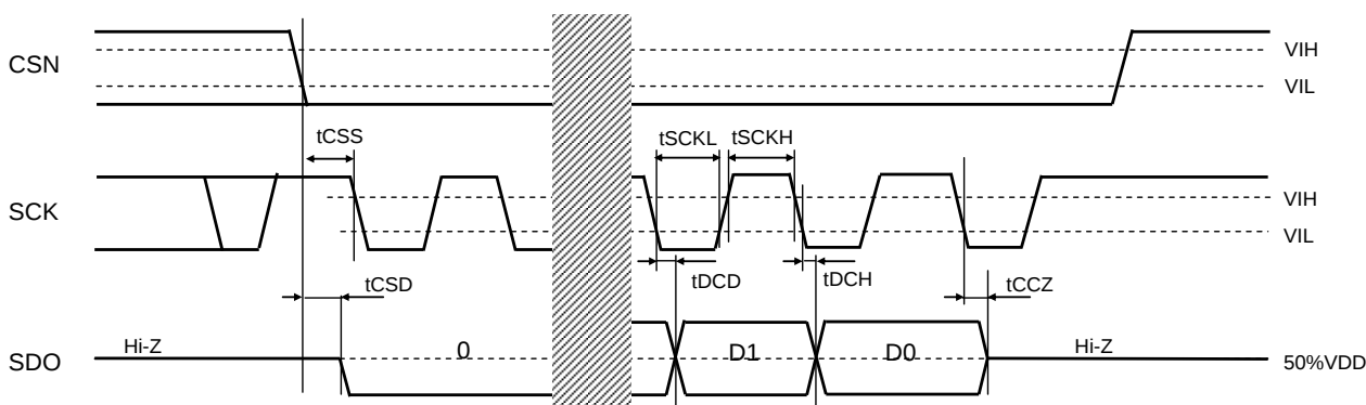
Figure 3. Data Output Timing 2
