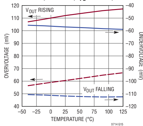
Power Good Thresholds vs Temperature ( V_{FB} - CTRL )
