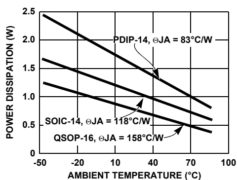
FIGURE 47. MAXIMUM POWER DISSIPATION vs AMBIENT TEMPERATURE QUADS ( T_{JMAX} = +150^{\circ}\text{C} )
