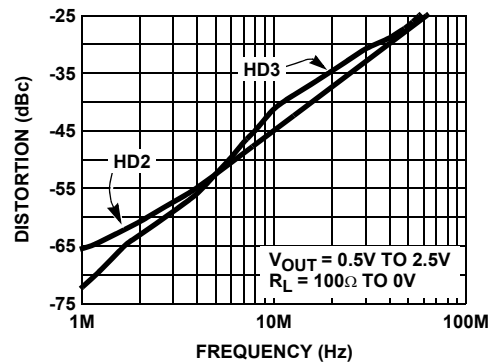
FIGURE 34. 2nd AND 3rd HARMONIC DISTORTION vs FREQUENCY
