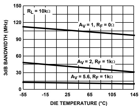
FIGURE 6. 3dB BANDWIDTH vs DIE TEMPERATURE FOR VARIOUS GAINS
