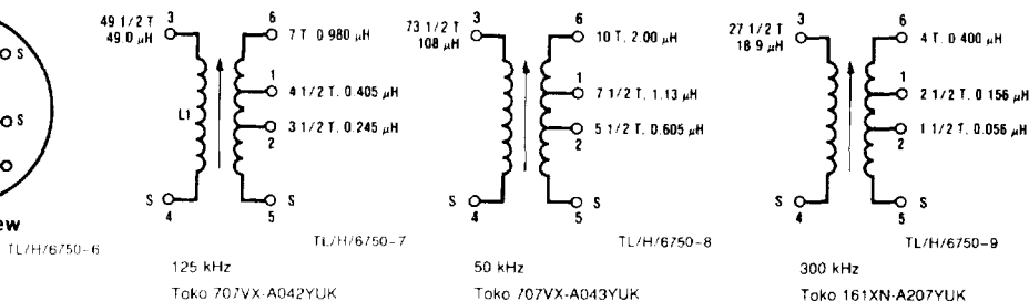
FIGURE 7. The recommended T_1 transformers, available through: Toko America, 1250 Feehanville Drive, Mount Prospect, IL, 60056, (312) 297-0070
