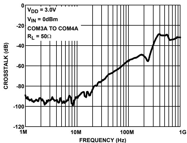
FIGURE 21. CROSSTALK
