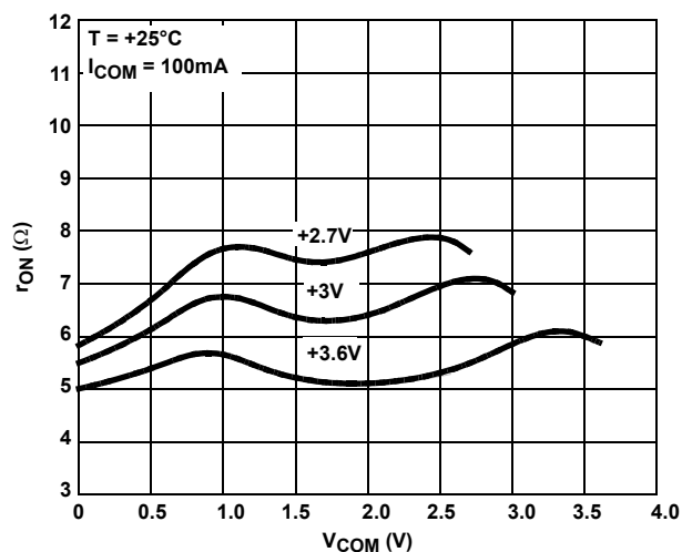
FIGURE 14. ON-RESISTANCE vs SWITCH VOLTAGE; COM1B AND COM4B
