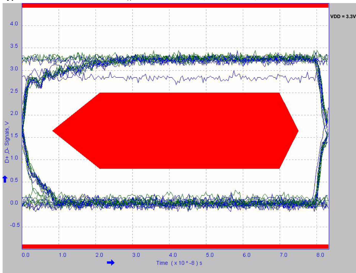
FIGURE 25. EYE PATTERN: 12Mbps; COM2x or COM3x SWITCH IN THE SIGNAL PATH
