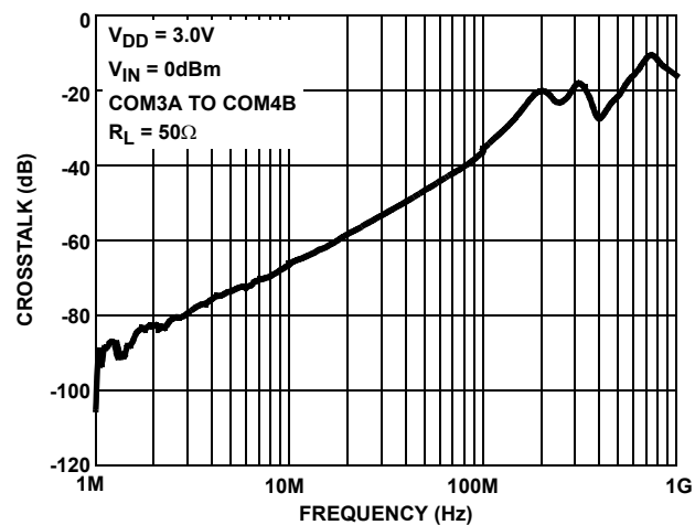
FIGURE 22. CROSSTALK
