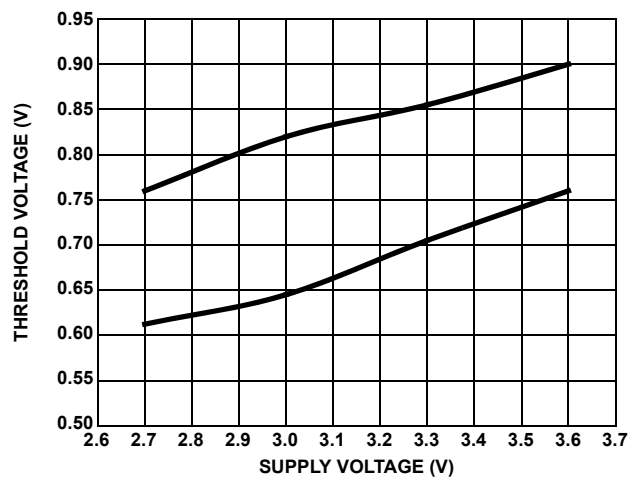
FIGURE 23. LOGIC INPUT THRESHOLD VOLTAGE vs SUPPLY VOLTAGE
