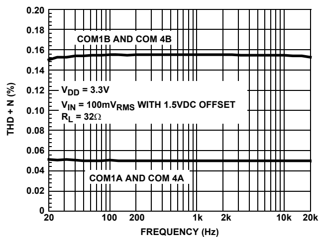
FIGURE 24. TOTAL HARMONIC DISTORTION vs FREQUENCY
