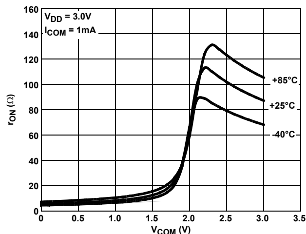
FIGURE 9. ON-RESISTANCE vs SWITCH VOLTAGE; COM2x AND COM3x
