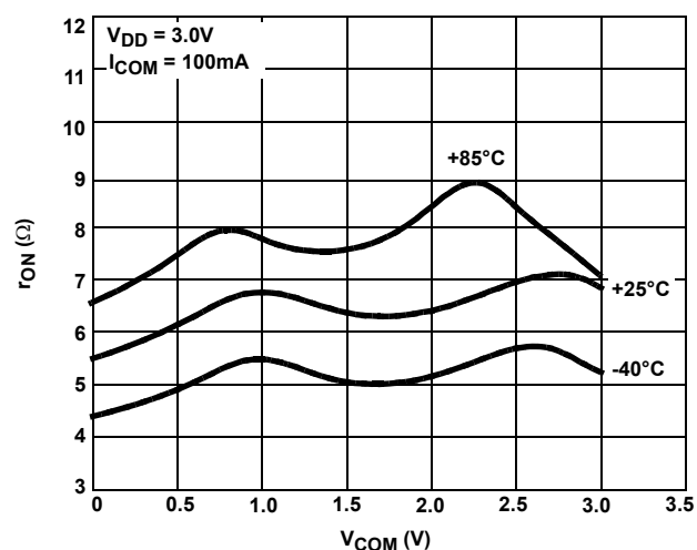
FIGURE 13. ON-RESISTANCE vs SWITCH VOLTAGE; COM1B AND COM4B
