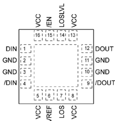
16-Pin QFN
