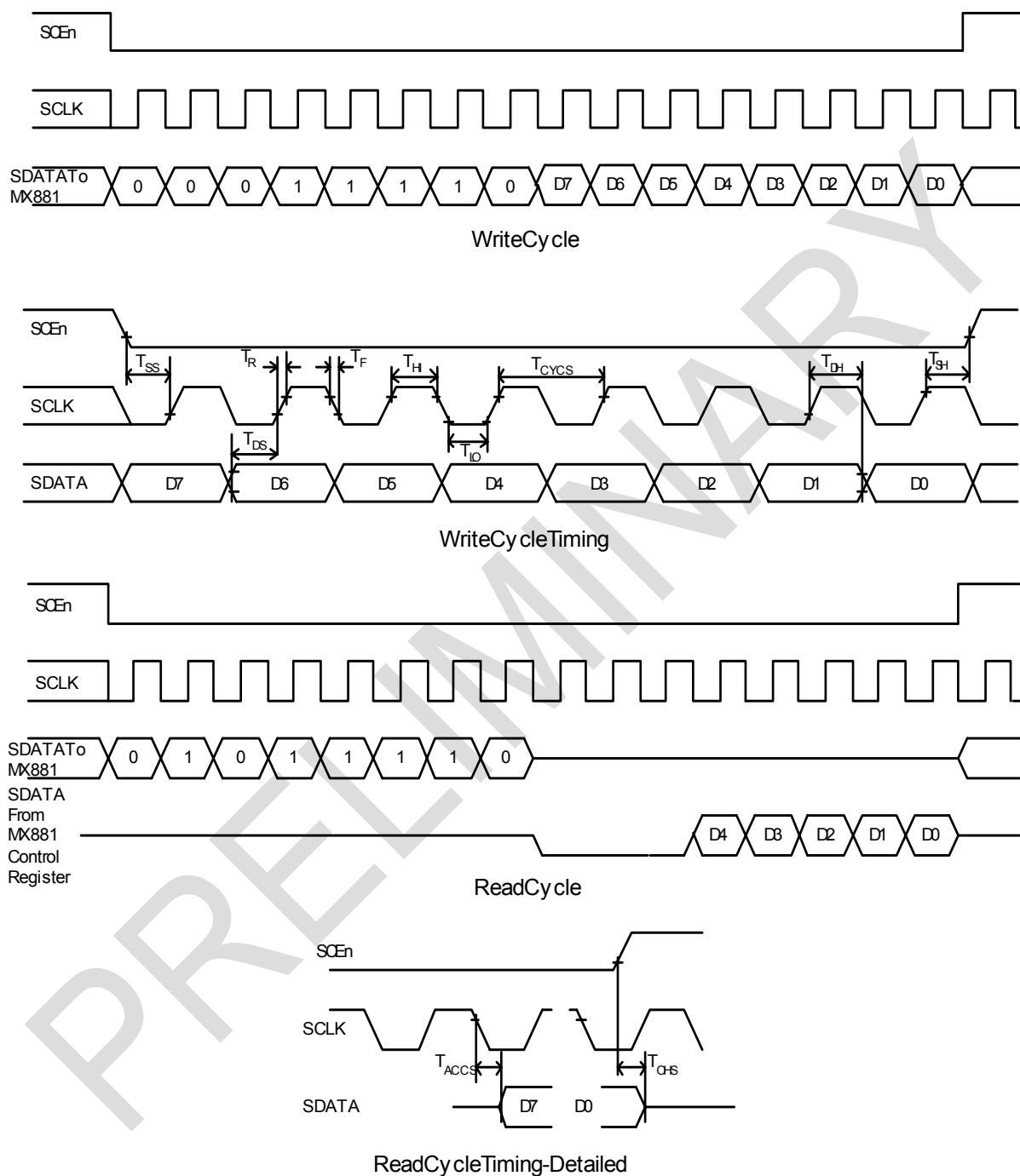
Figure 3 – 3-WIRE SPI
