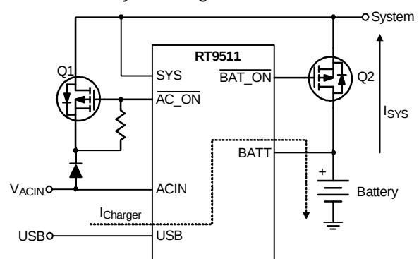
Figure 4. USB Input
