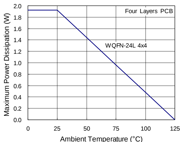
Figure 9. Derating Curves for RT9511 Packages
