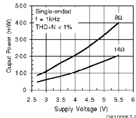
Output Power vs Supply Voltage Single-Ended
