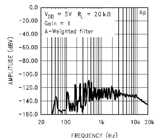
Microphone Noise Floor
