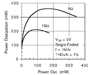
Power Dissipation, Single-Ended
