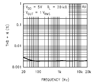
Equalizer Output THD+N vs Frequency
