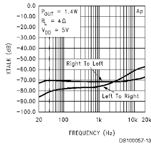
Power Amplifier Crosstalk, Bridged
