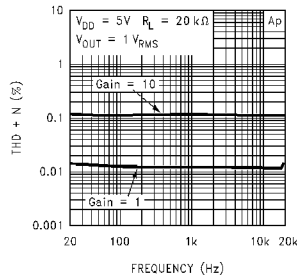
Microphone THD+N vs Frequency
