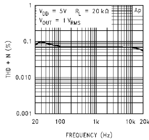
Line Out THD+N vs Frequency
