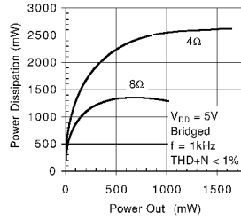
Power Dissipation, Bridged
