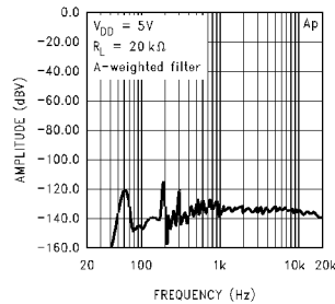
Line Out Noise Floor
