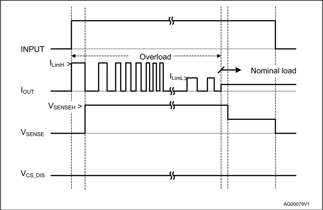
Figure 13. Intermittent overload
