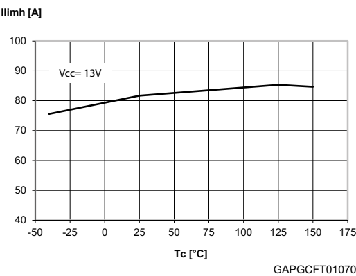
Figure 27. I_{LIMH} vs T_{case}
