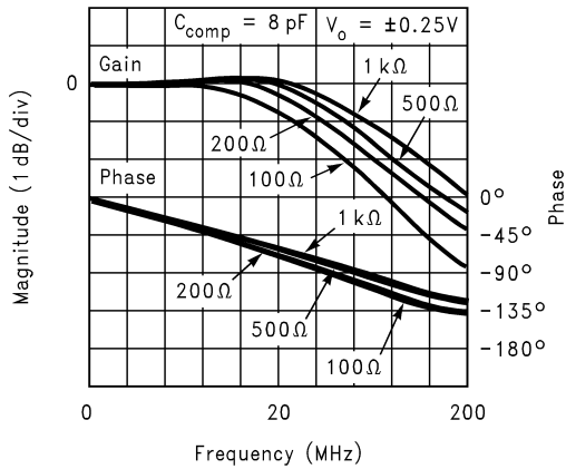
Small Signal/Phase vs. Load
