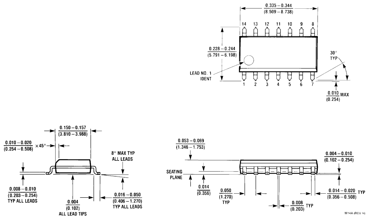
NS Package Number M14A
