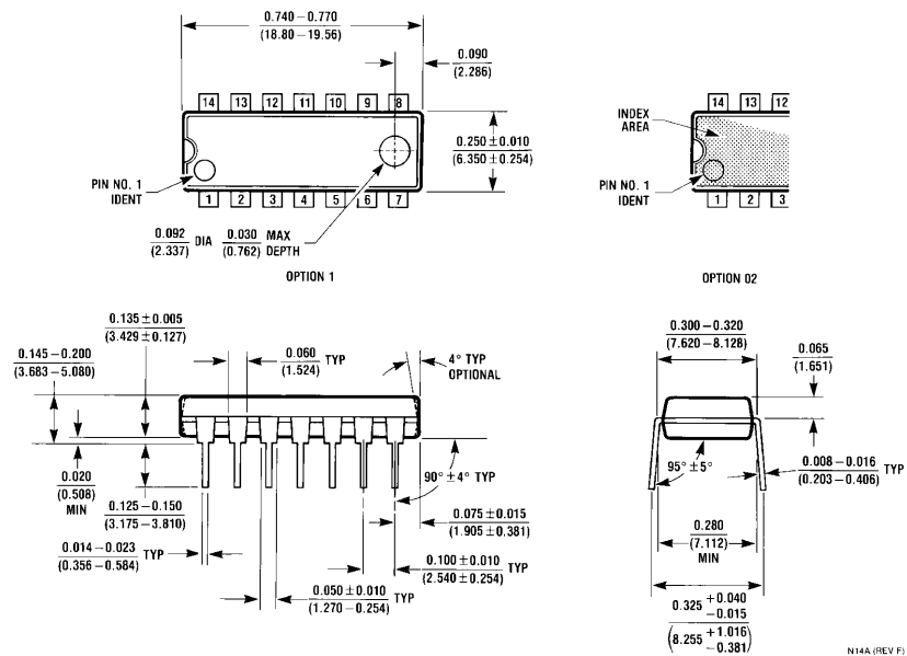
NS Package Number N14A
