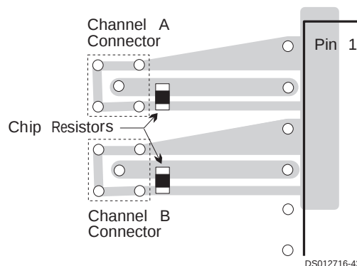
FIGURE 6. Alternate Layout Using Guard Ring
