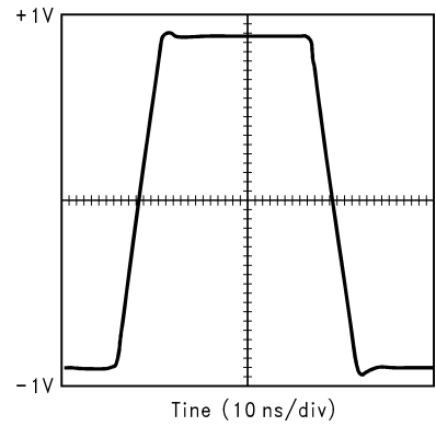
Digitized Pulse Response
