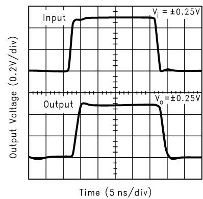
Small Signal Pulse Response
