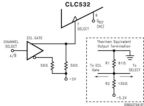
FIGURE 2. ECL Level Channel SELECT Configuration
