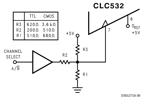
FIGURE 3. TTL/CMOS Level Channel SELECT Configuration
