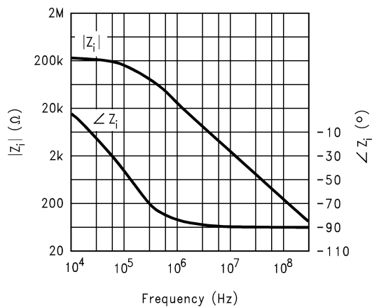
Input Impedance
