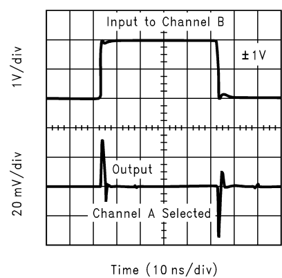
Transient Isolation
