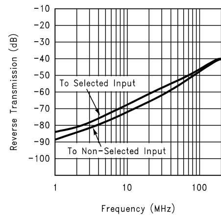
Reverse Transmission ( S_{12} )
