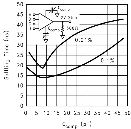
Settling Time vs C_{comp}
