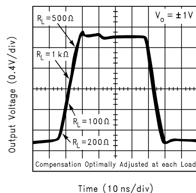
Large Signal Pulse Response vs. R_L
