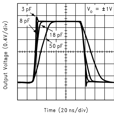
Large Signal Pulse Response vs. C_{comp}
