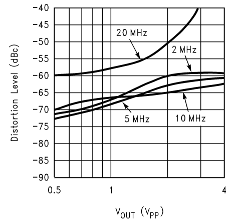
2nd Harmonic Distortion vs. V_{OUT} ; R_L = 100\Omega
