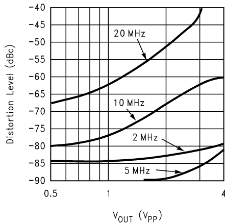
2nd Harmonic Distortion vs. V_{OUT} ; R_L = 500\Omega
