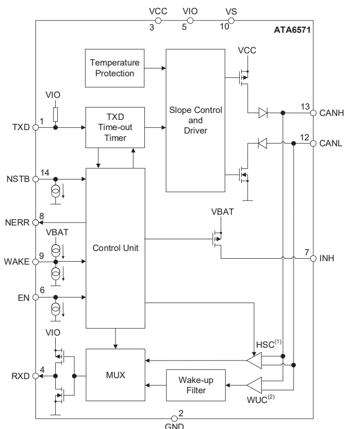
Figure 1. Simplified Block Diagram
