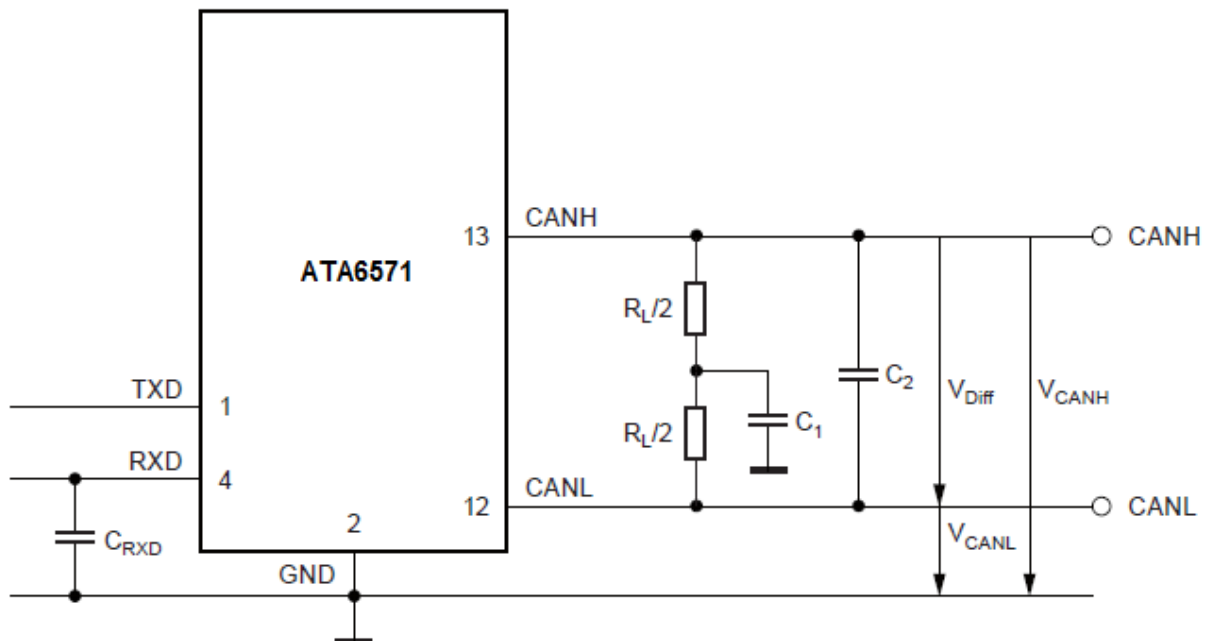
Figure 6-3. Test Circuit
