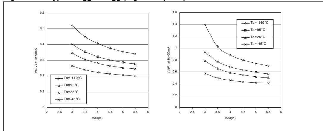
Figure 74. Typical V_{OL} vs. V_{DD} (high-sink ports)
