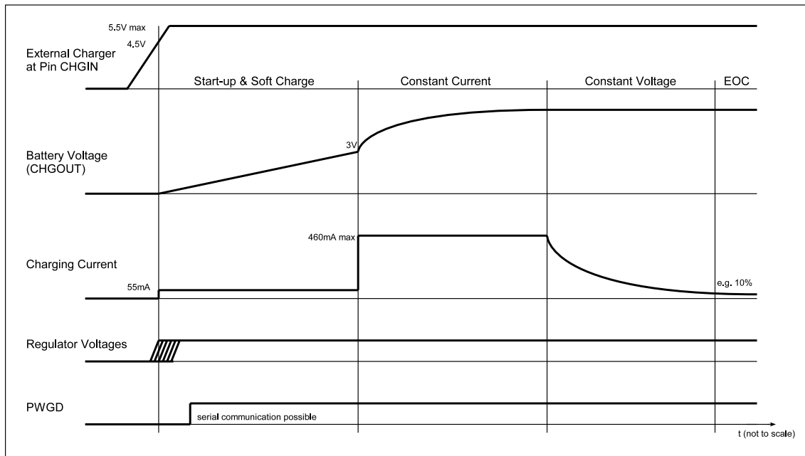
Figure 28. Charger States
