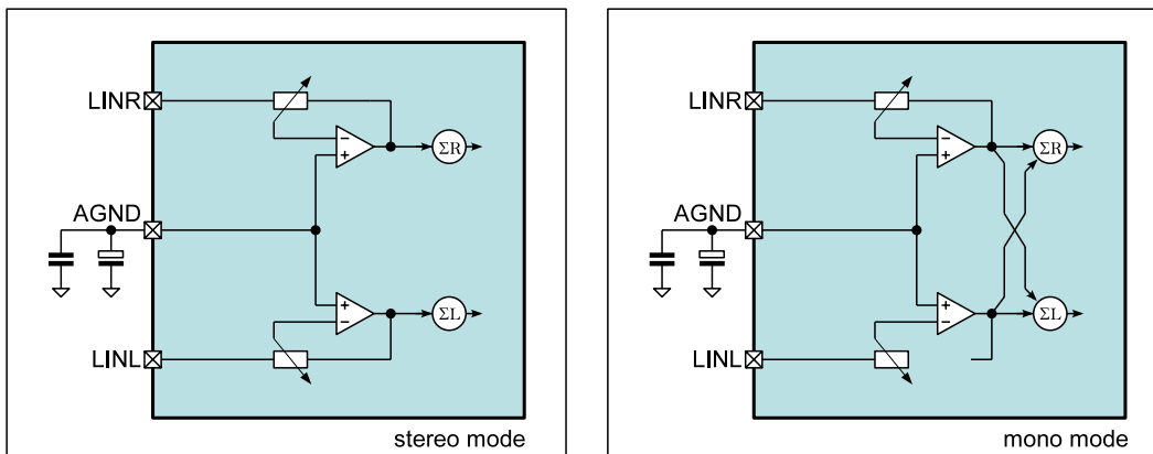
Figure 3. Line Inputs
