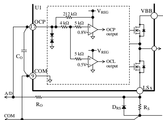
Figure 10-20. Internal Circuit Diagram of OCP Pin
