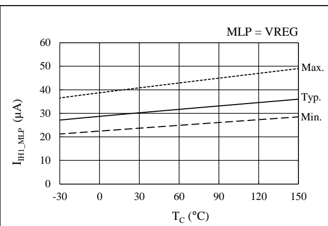
Figure 13-10. MLP Pin High Level Input Current, I_{IH1\_MLP} vs. T_C
