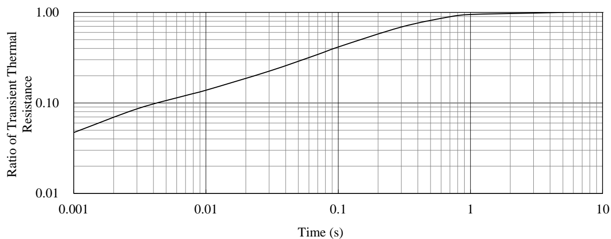
Figure 13-1. Transient Thermal Resistance: SX68126M / SX68127M
