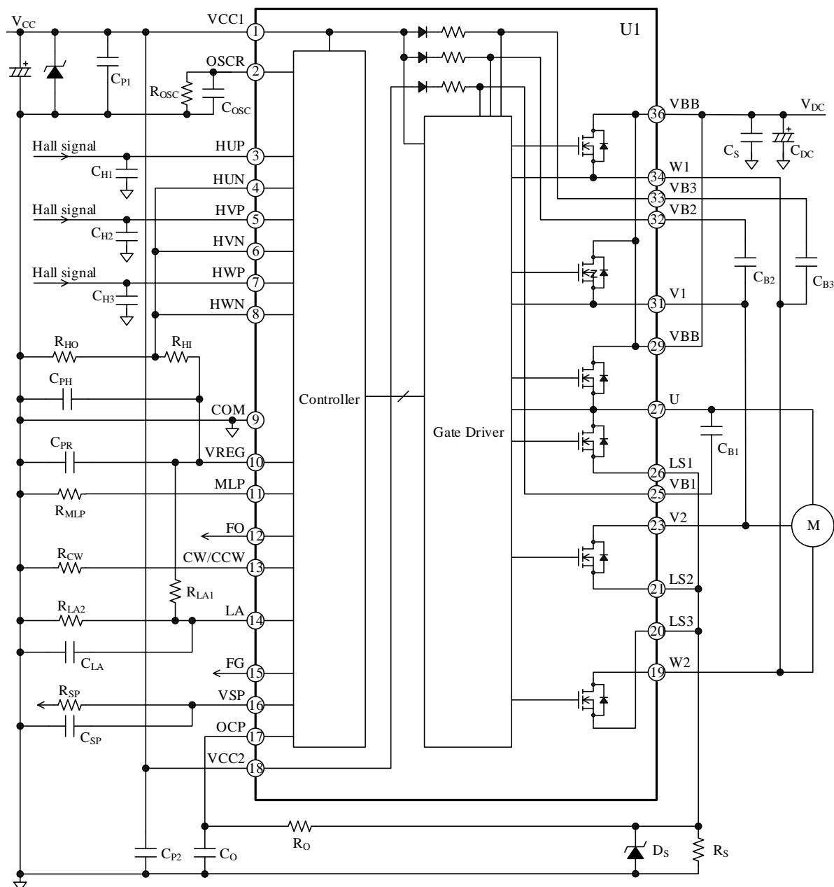
Figure 7-2. Application Using Signals Input from Hall ICs
