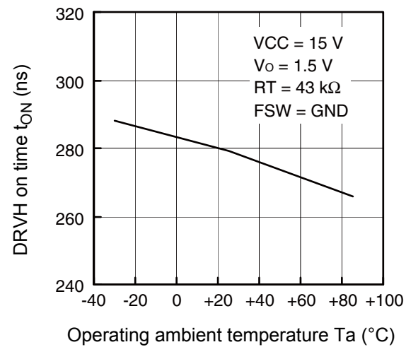
DRVH on time vs. Operating ambient temperature
