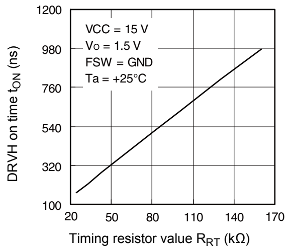
DRVH on time vs. Timing resistor value
