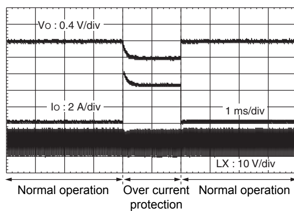
Output Over Current Waveform (UVP Disabled)
