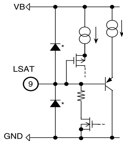
<<Output block (OUT-2)>>
