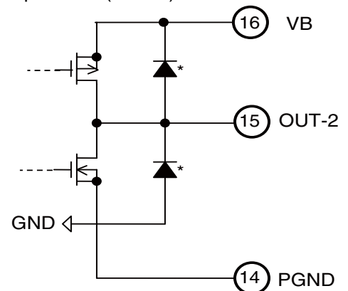
<<Output block (OUT-2)>>
