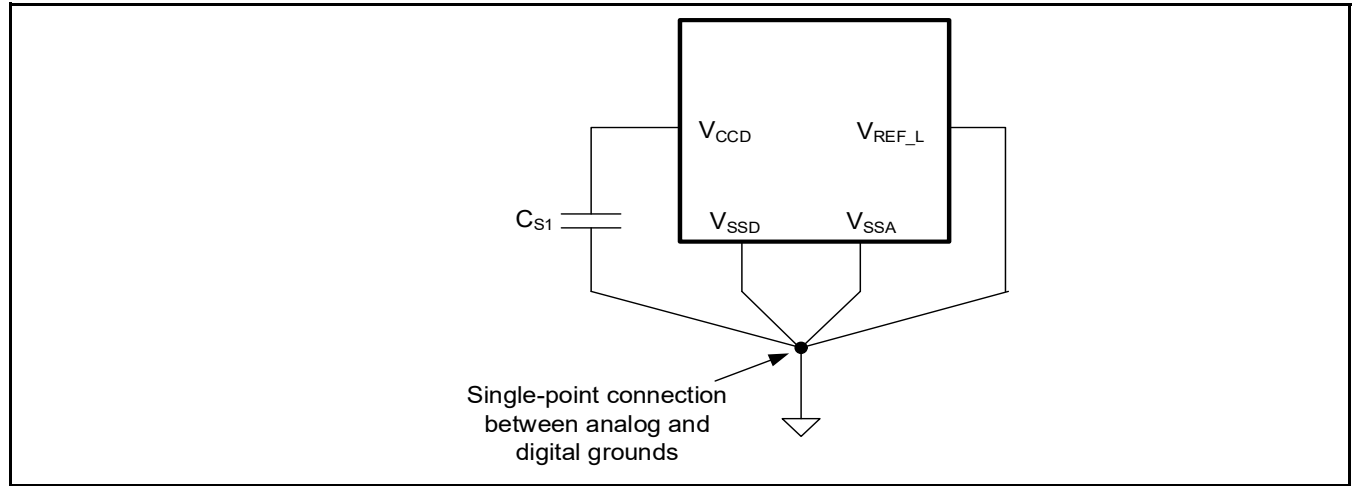
Figure 26-2 Smoothing capacitor
