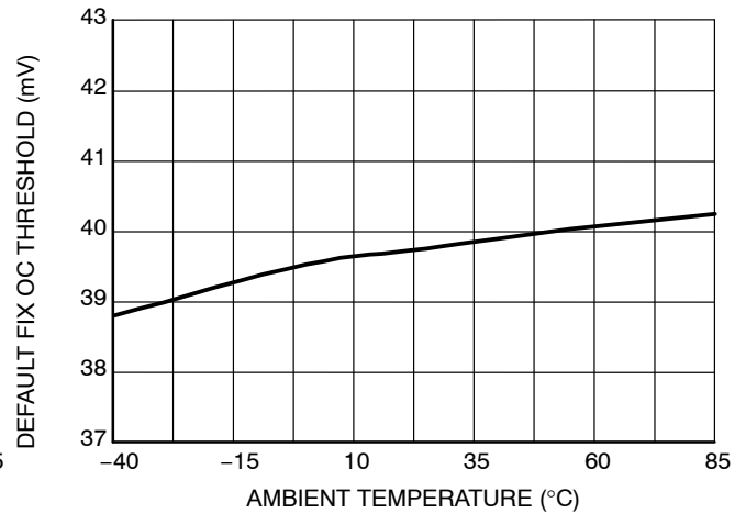
Figure 8. Default Fix OC Threshold vs Ambient Temperature
