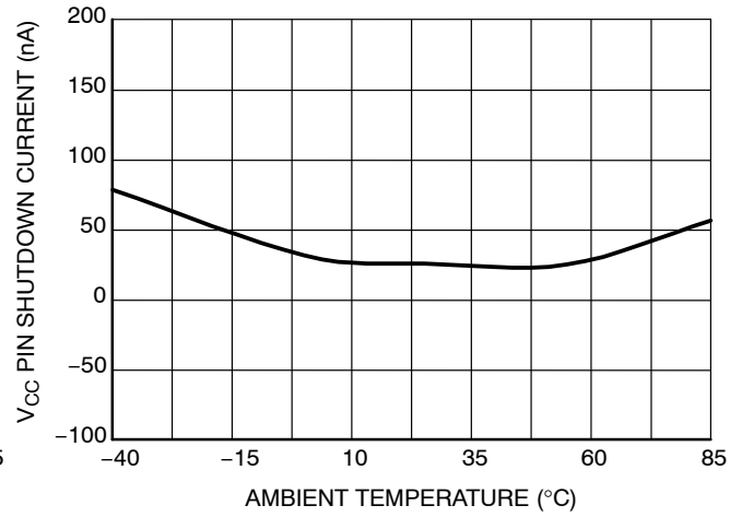
Figure 4. V CC Shutdown Current vs Ambient Temperature
