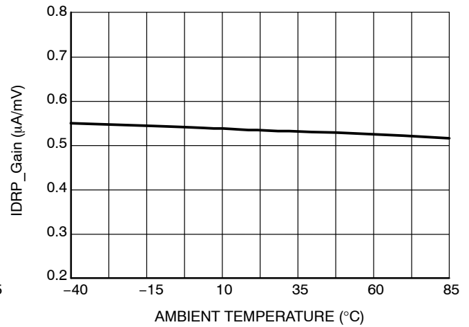
Figure 6. IDRP Gain vs Ambient Temperature
