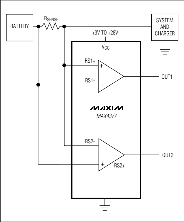
Figure 2. Bidirectional Current Monitor
