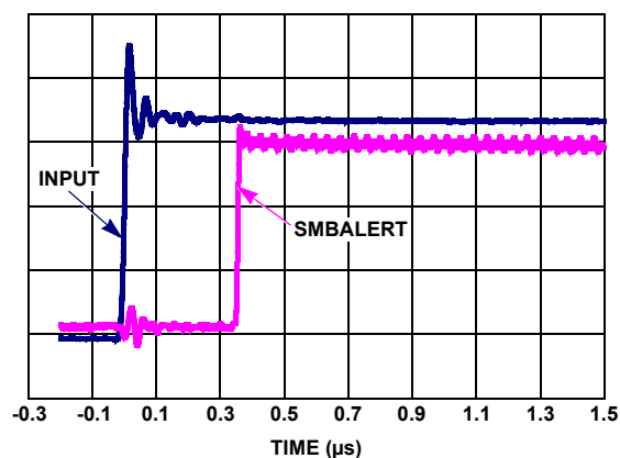
FIGURE 86. OV OR UV OR OC ALERT RESPONSE TIME
