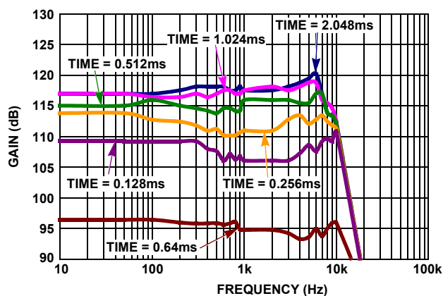
FIGURE 110. CMRR vs FREQUENCY
