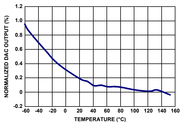
FIGURE 82. NORMALIZED DAC OUTPUT vs TEMPERATURE
