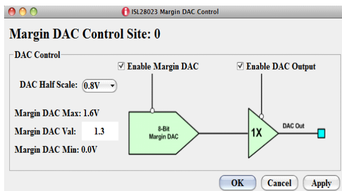
FIGURE 103. SIMPLIFIED BLOCK DIAGRAM OF THE MARGIN DAC FUNCTIONS WITHIN THE DPM
