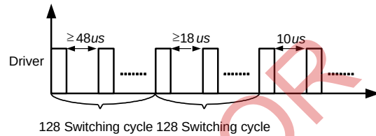
Figure 2— \tau_{\text{min off}} at start-up
